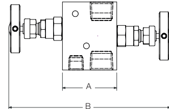
Example shown: 2-valve manifold with integral A-LOK® connections.
