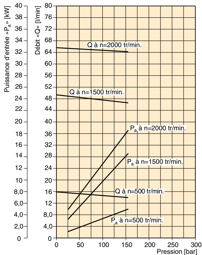
PGP 511 - 33,0 cm 3
