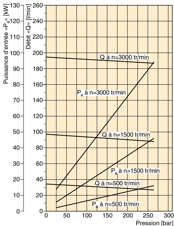
PGP640 - 65,0 cm 3
