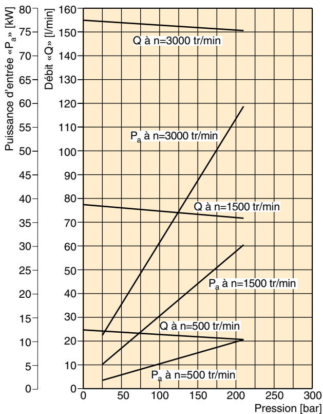
PGP 620 - 52,0 cm 3
