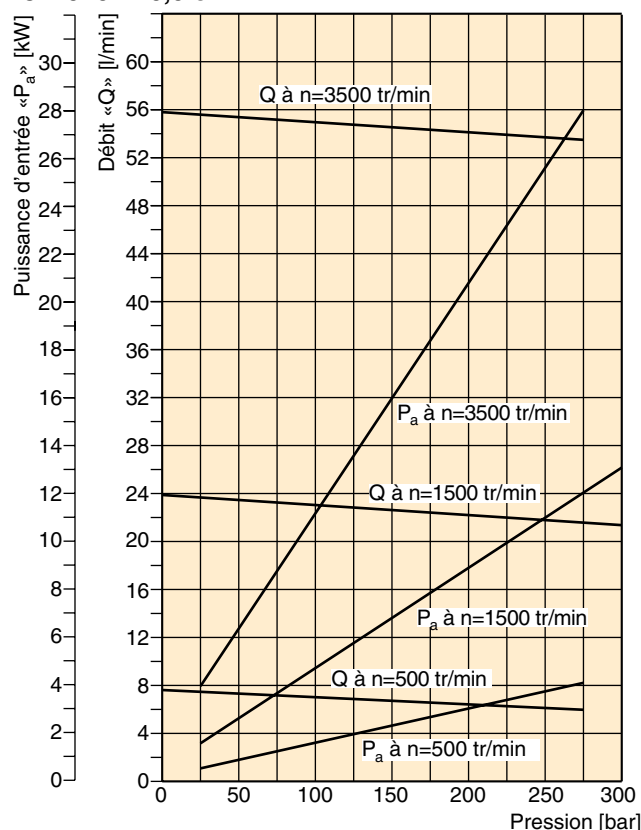
PGP 620 - 41,0 cm 3
