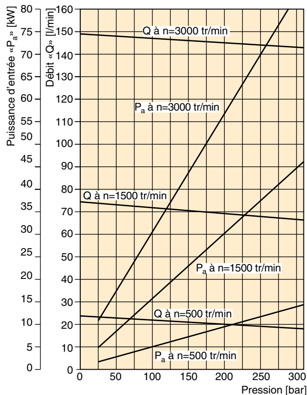
PGP640 - 50,0 cm 3
