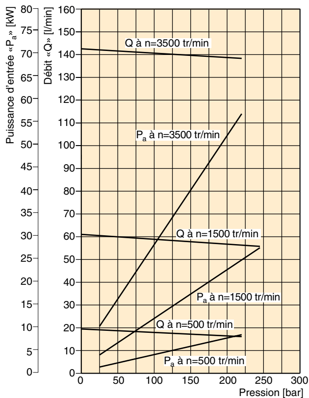
PGP 620 - 41,0 cm 3
