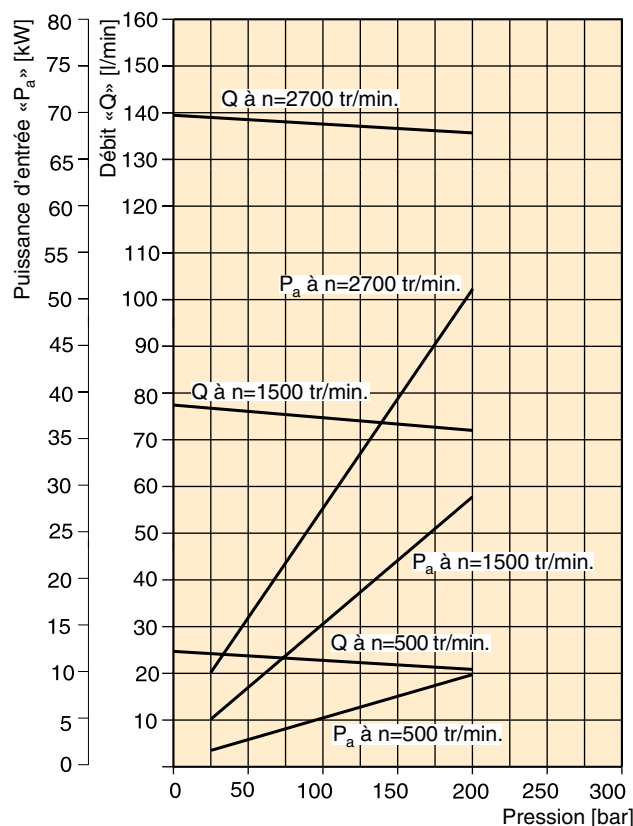
PGP 517- 52,0 cm 3
